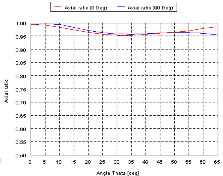
Axial ratio
