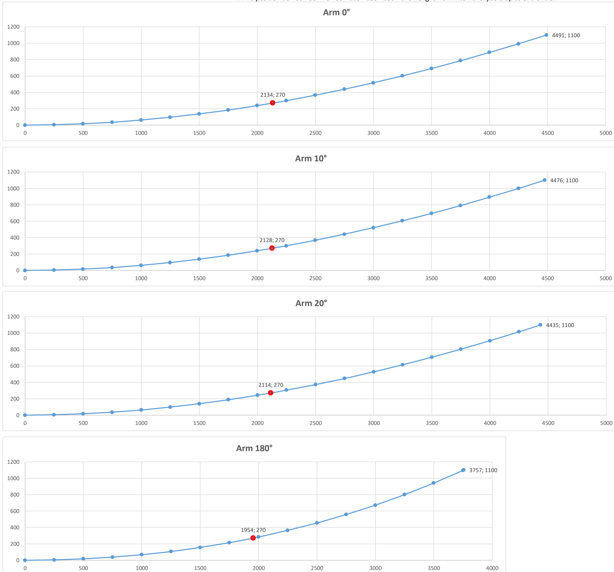
Arms position 0 - 20 - 40 - 60 - 80 - 100 - 120 - 140 - 160 - 180° full length Arms position 10 - 30 - 50 - 70 - 90 - 110 - 130 - 150 - 170° length from internal ellipsoid up to end of dish
